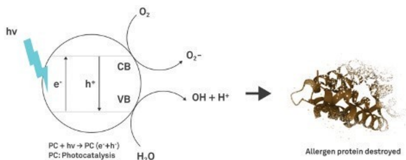
Fig. 1. PECO mechanism on the destruction of allergen proteins.
